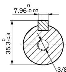
Shaft G: Cylindrical shaft \varnothing 31.75 Parallel key 7.96 \times 7.96 \times 31.75
