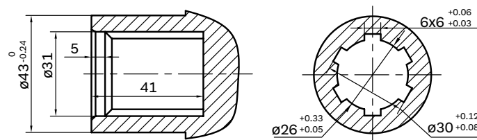
SHAFT N
