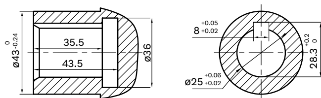
SHAFT A
