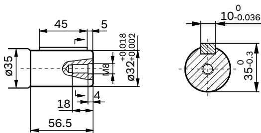
Shaft B:
