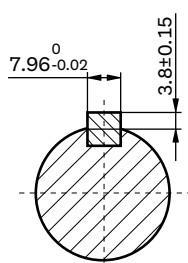
Shaft T4: Cone-shaft \varnothing 31.75 Parallel key 7.96 \times 7.96 \times 25.4 Tightening torque: 200 \pm 10 \text{ Nm}
